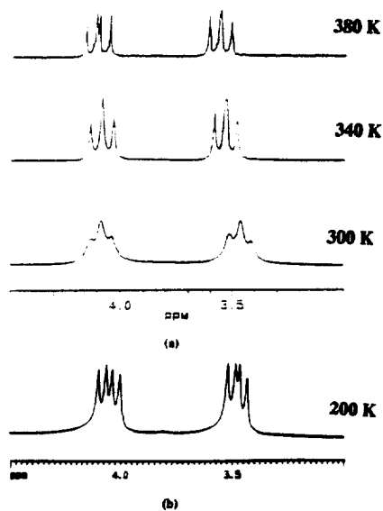
Figure 4. Variable temperature ^1\text{H} NMR spectra of 6by , methylene region: a) 300 MHz, \text{Cl}_2\text{CD}-\text{CDCl}_2 and b) 400 MHz, \text{CD}_2\text{Cl}_2 .
