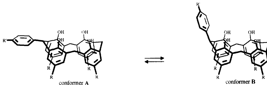
Figure 2. Conformational equilibrium for calix[4]arenes 4 .
