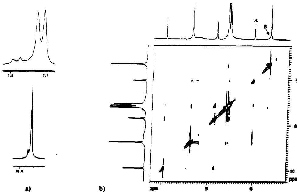
Figure 6. ^1\text{H} NMR (400 MHz, \text{CD}_2\text{Cl}_2 ) of 6by at 200 K: a) parts of the 1D spectrum; b) 2D-NOESY map.
