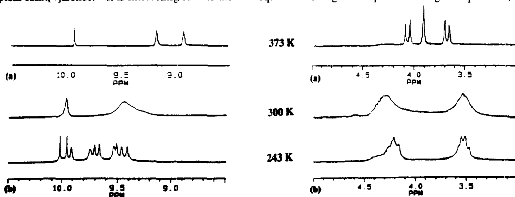
Figure 3. Variable temperature 1 H NMR spectra of 4by [300 MHz, \text{Cl}_2\text{CD}-\text{CDCl}_2 (a), \text{CDCl}_3 (b)]: methylene region (on the right) and hydroxylic region (on the left).
