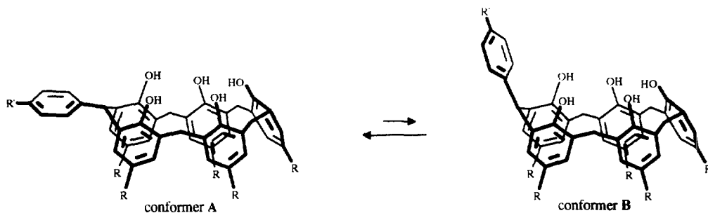
Figure 5. Conformational equilibrium for calix[5]arenes 6 .
